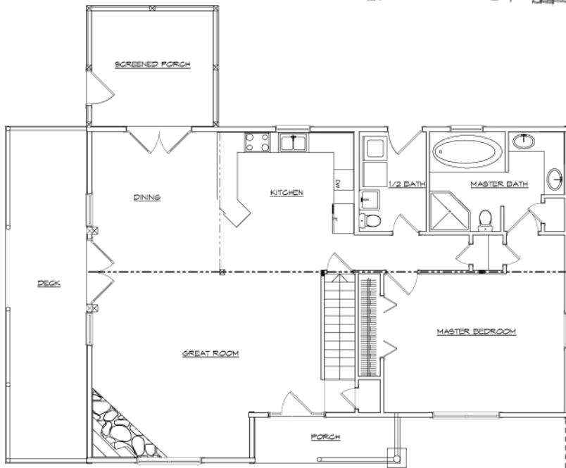
MAIN FLOOR
