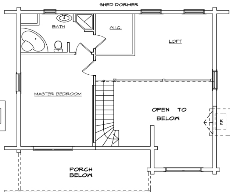
SECOND FLOOR
